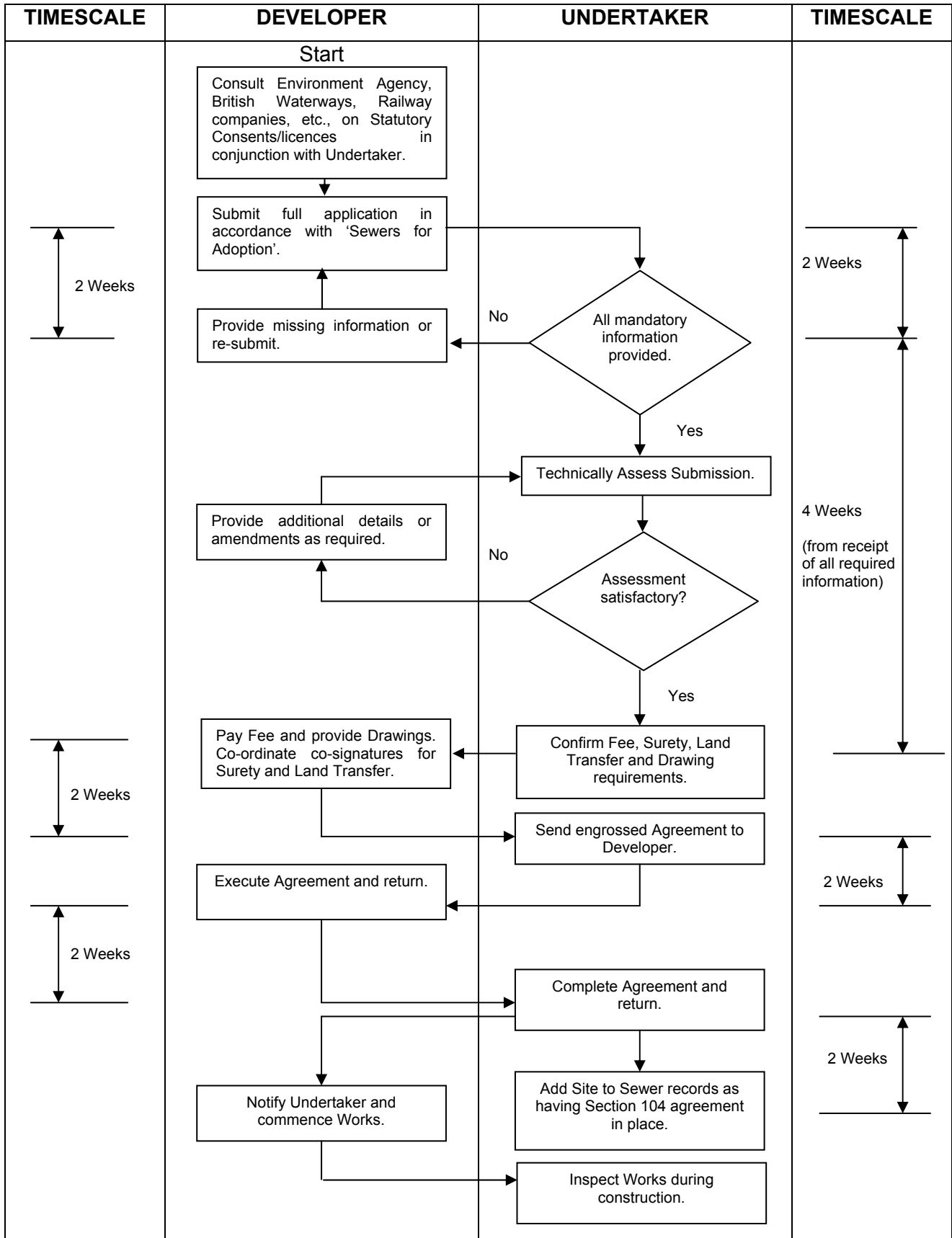
Figure 1.1 Quick Reference Flowchart (Application to Start On-Site)
